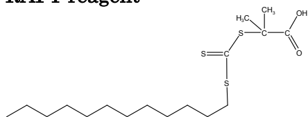
2-dodecylsulfanyl-2-methylpropionic acid
